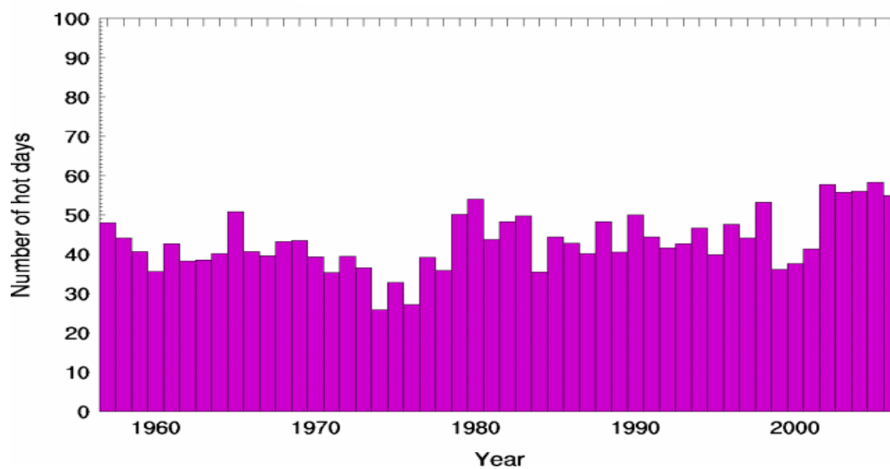
Figure 1: Average number of hot days in Australia over 30 years
