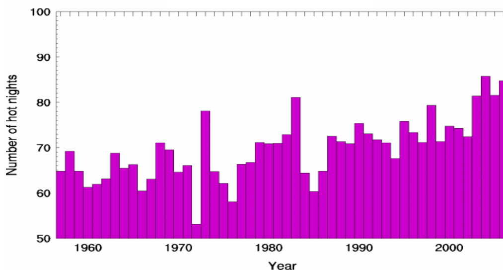
Figure 2: Average number of hot nights in Australia over 30 years
